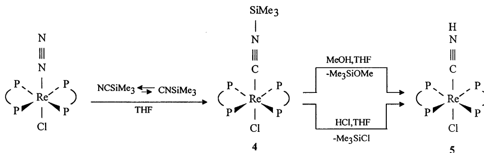
Scheme 3. Syntheses of the \text{CNSiMe}_3 and \text{CNH} diphosphinic complexes of Re(I) [9,10].
