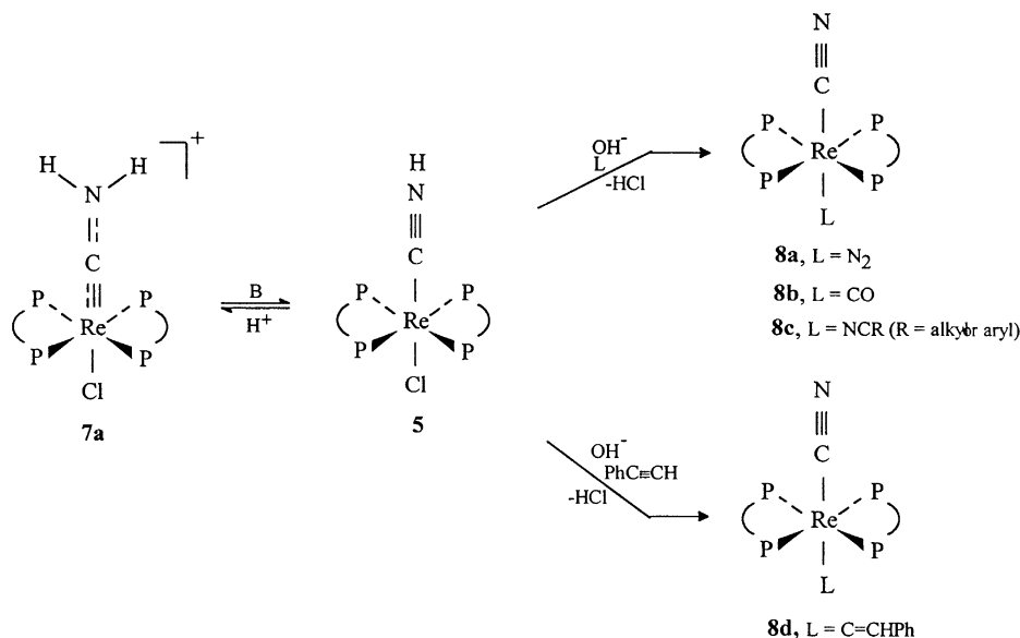
Scheme 5. Conversion of the aminocarbyne complex 7a into Re cyano-complexes of dinitrogen, carbonyl, organonitriles or phenylvinylidene: B = NEt 3 or NBu 4 OH [30].
