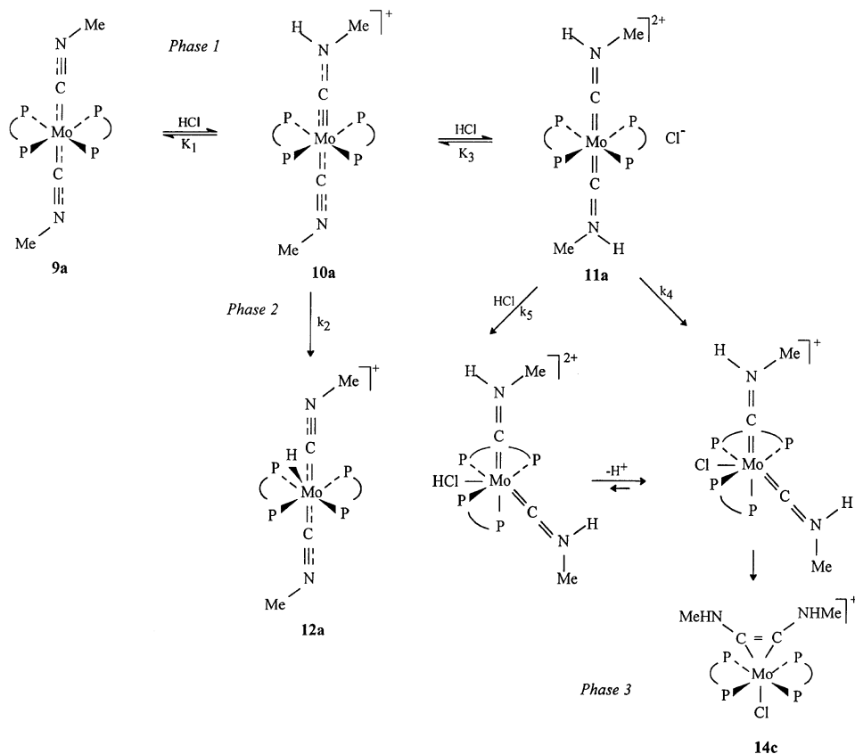
Scheme 13. Mechanisms of protonation of the di(methylisocyanide) complex trans -[Mo(CNMe) 2 (dppe) 2 ] ( 9a ) to give aminocarbynes, hydride and (diamino)acetylene products [56].
