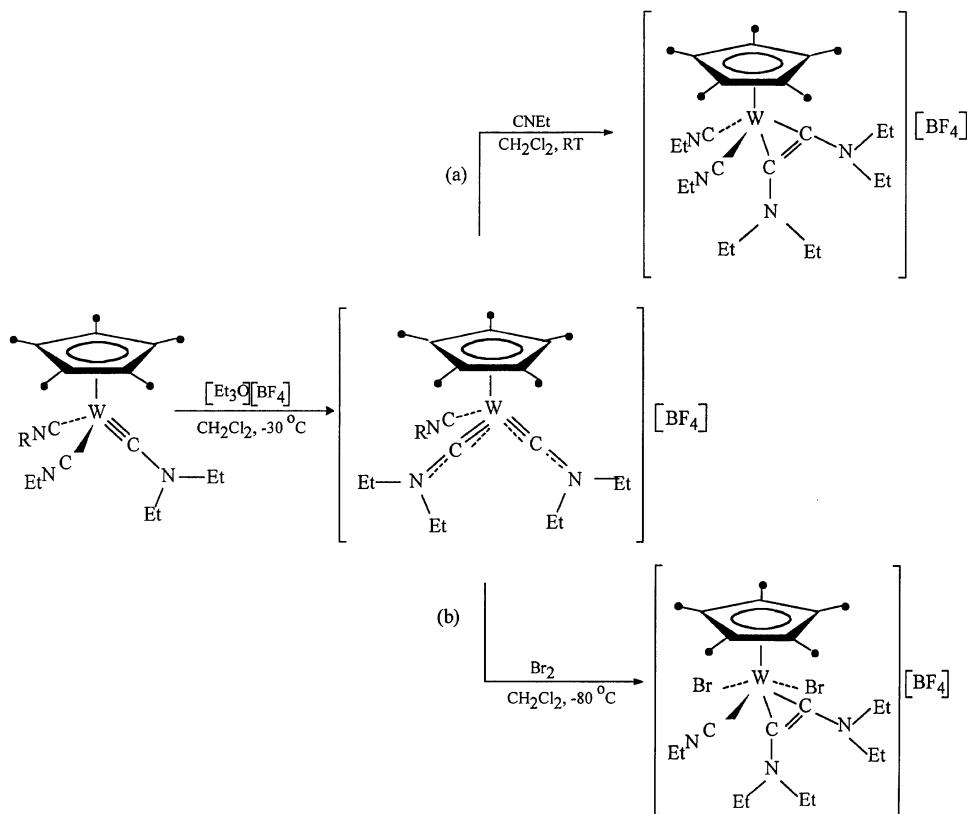
Scheme 12. Coupling of aminocarbyne ligands promoted by: (a) a nucleophilic addition or (b) an oxidative addition reaction [49a,b].
