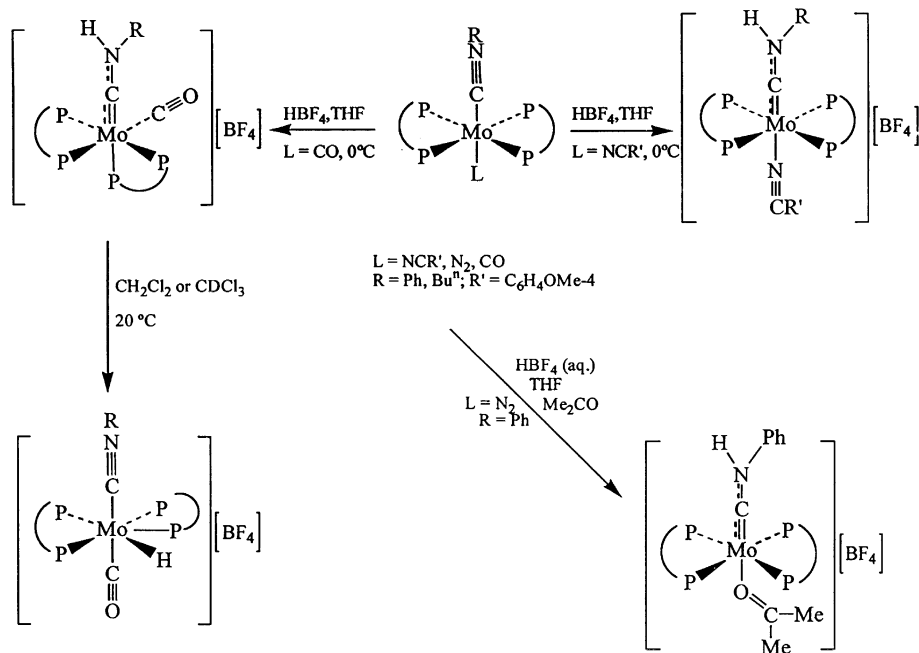
Scheme 7. Protonation of mono(isocyanide) phosphinic complexes of Mo(0) to give aminocarbyne products [42].
