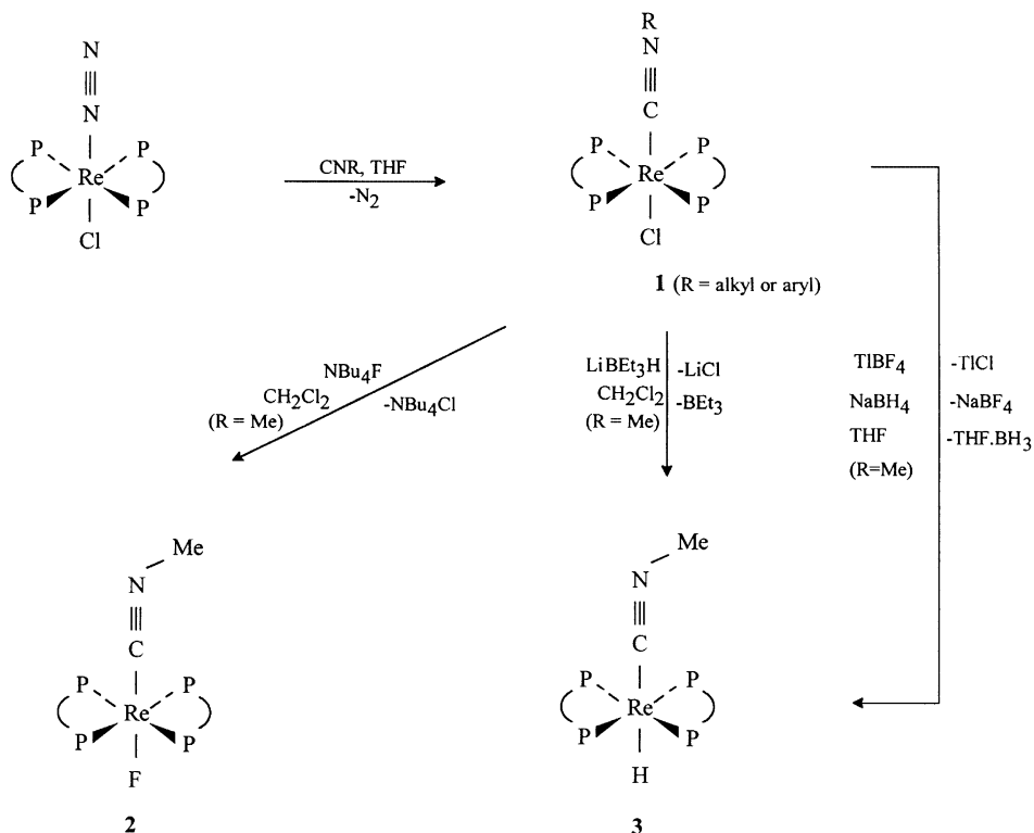
Scheme 2. Syntheses of alkyl- and aryl-isocyanide diphosphinic complexes of Re(I) [3,4,7,8]. \text{dppe} = \text{Ph}_2\text{PCH}_2\text{CH}_2\text{PPh}_2 .
