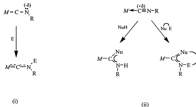
Scheme 1. Activation of isocyanide towards (i) electrophilic and (ii) nucleophilic additions: M — transition metal coordination centre; E — electrophile; NuH — protic nucleophile; \overset{+}{Nu}E — nucleophile which also bears an electrophilic centre.
