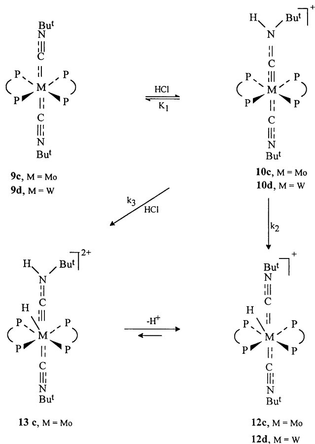
Scheme 15. Mechanism of protonation of the di( tert -butylisocyanide) complexes trans -[M(CN t Bu) 2 (dppe) 2 ] ( 9c , M = Mo; 9d W) to give aminocarbene, hydride and hydride–aminocarbene products [56].
